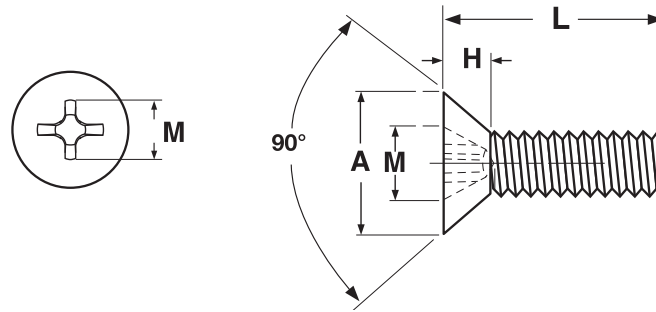
DIN 965 90° FLAT PHILLIPS (TYPE H RECESS) MACHINE SCREWS
