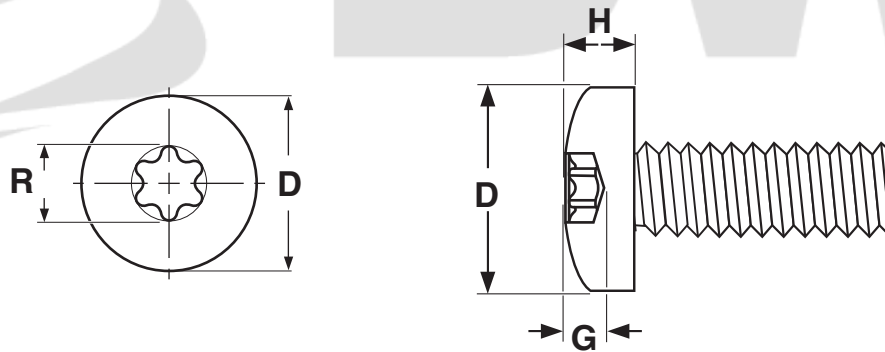
METRIC - ISO 7045 Six-LOBE PAN HEAD MACHINE SCREWS
