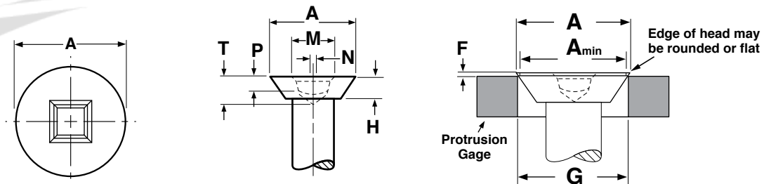
FLAT UNDERCUT SQUARE RECESS HEADS FOR TAPPING SCREWS
