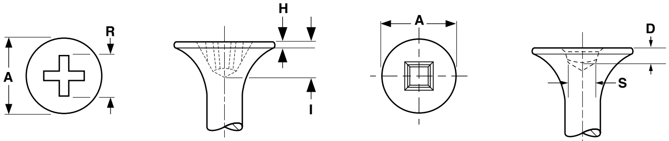
BUGLE HEADS FOR DRYWALL, PARTICLE BOARD & DECK SCREWS
