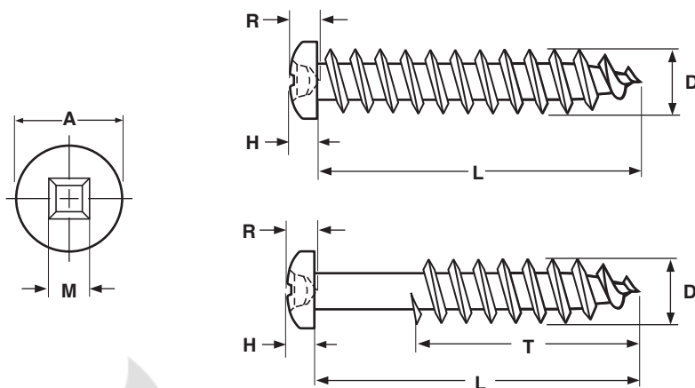
PAN SQUARE RECESS DEEP THREAD WOOD SCREW
